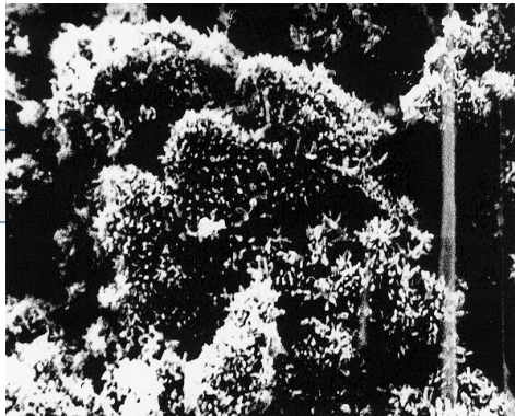
\text{PbO}_2
